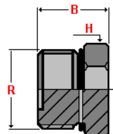
35.141. - Straight Thread Plug
